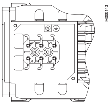
Motor sizes 56-80.
